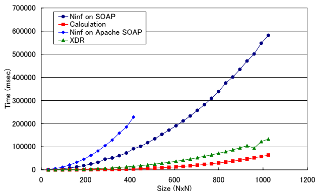
Figure 8. Performance of Ninf-on-SOAP (WAN)
