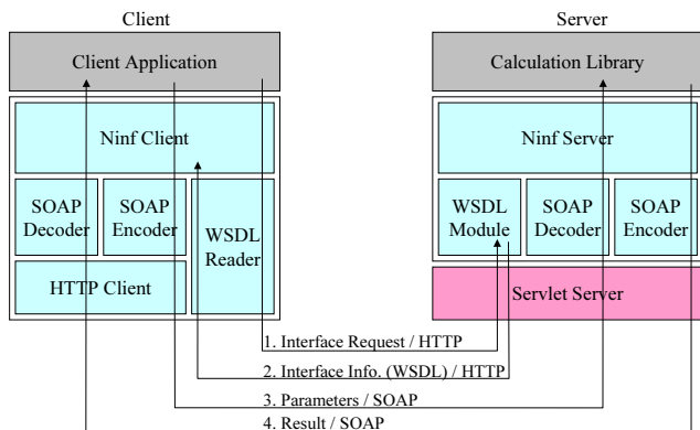
Figure 6. Ninf-on-SOAP architecture
