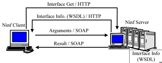
Figure 2. SOAP-based GridRPC system architecture
