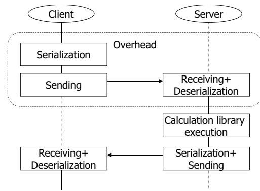
Figure 9. Ninf-on-SOAP execution flow
