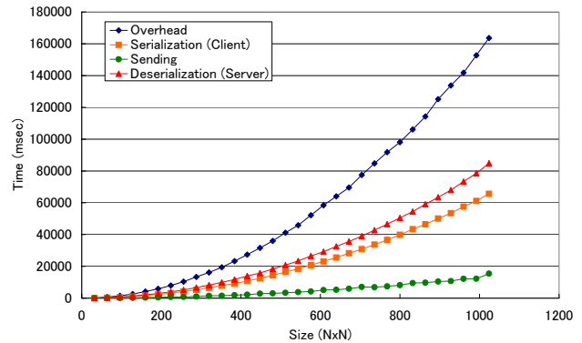
Figure 10. Detailed overhead analysis (LAN)
