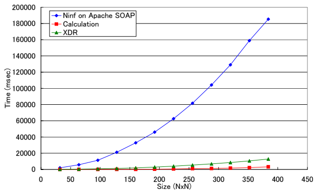
Figure 5. Ninf on Apache SOAP performance (WAN)
